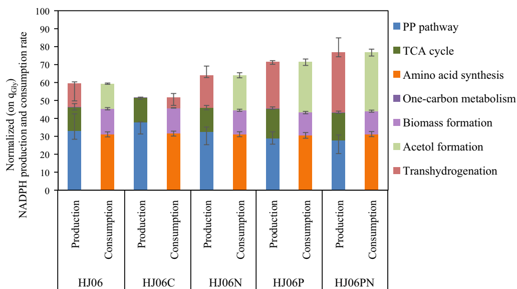
Fig. 3 Estimated production and consumption of NADPH by acetol-producing and non-producing E. coli strains. q_{gly} , the specific glycerol consumption rate
