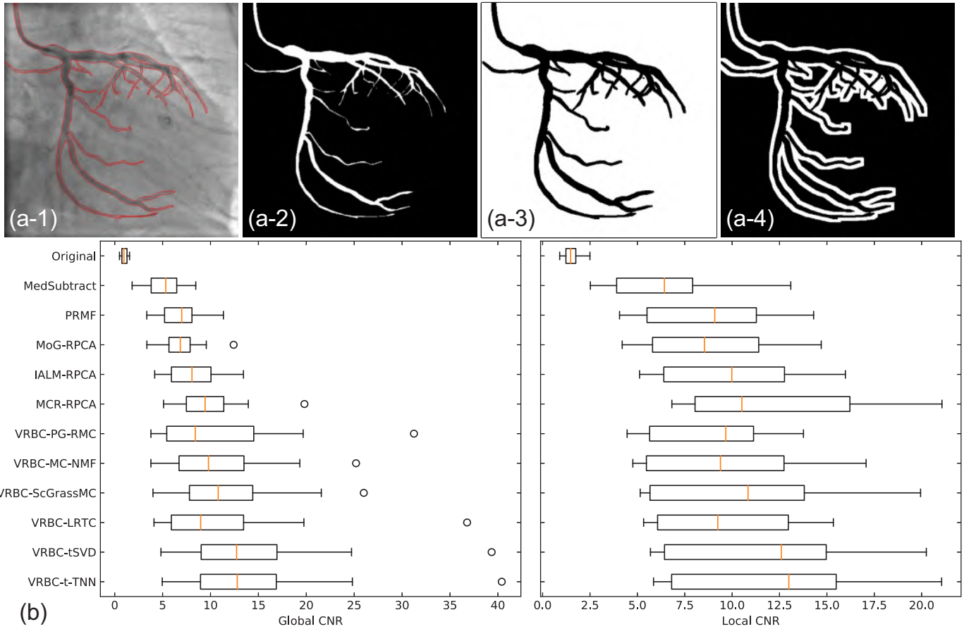
Fig. 9. CNR values on real data. (a-1)–(a-4) Original image with manually drawn vessel edges, the vessel regions, the global background regions, and the local background regions. (b) Global and local CNR values of twelve images from different image sequences of real data.
